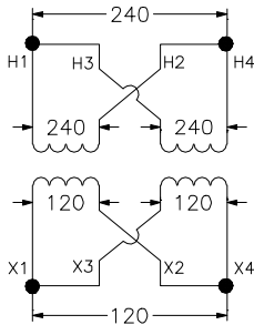
PARALLEL CONNECTION
