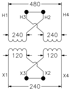
SERIES CONNECTION
