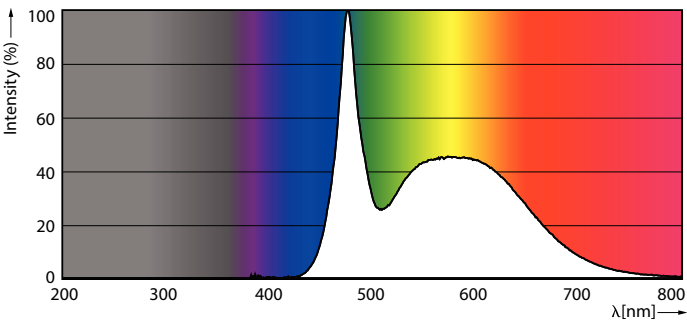
Spectral Power Distribution Colour - Ess LEDBulb 12-100W E27 6500K 4PF/6 MX
