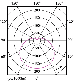
Light Distribution Diagram - Ess LEDBulb 12-100W E27 6500K 4PF/6 MX
