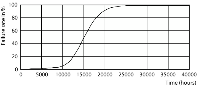
Life Expectancy Diagram - Ess LEDBulb 8-60W E27 6500K 4PF/6 MX
