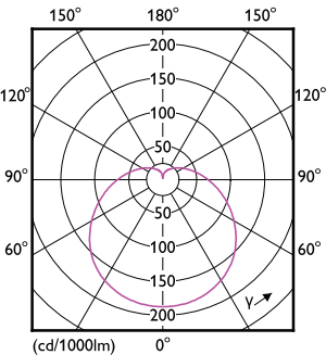
Light Distribution Diagram - Ess LEDBulb 8-60W E27 6500K 4PF/6 MX
