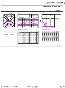
General uniform lighting - Ess LEDBulb 8-60W E27 6500K 1PF/6 MX
