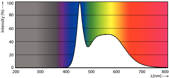
Spectral Power Distribution Colour - Ess LEDBulb 8-60W E27 6500K 1PF/6 MX
