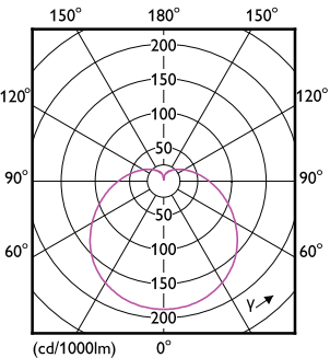
Light Distribution Diagram - Ess LEDBulb 8-60W E27 6500K 1PF/6 MX
